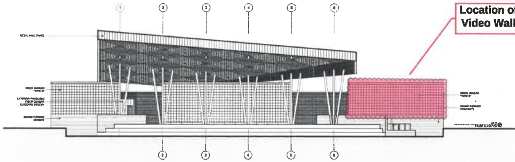
A1 SOUTH ELEVATION
